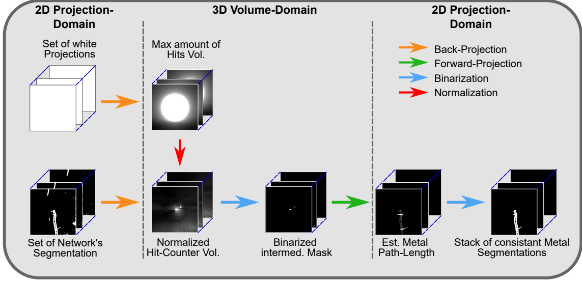
Figure 3: Illustration of the single steps of the Consistency Filter post-processing.
