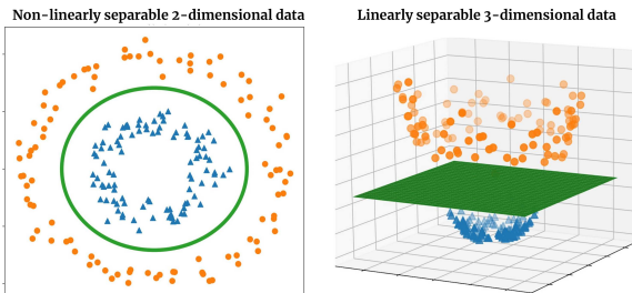
Figure 1: Data that is only non-linearly separable in lower dimensions can become linearly separable in higher dimensions, illustrated here for a simple case of 2-dimensional data that becomes linearly separable when lifted into 3-dimensions. This is the underlying principle in kernel based methods and tensor networks which learn linear decision boundaries in high dimensional spaces.
